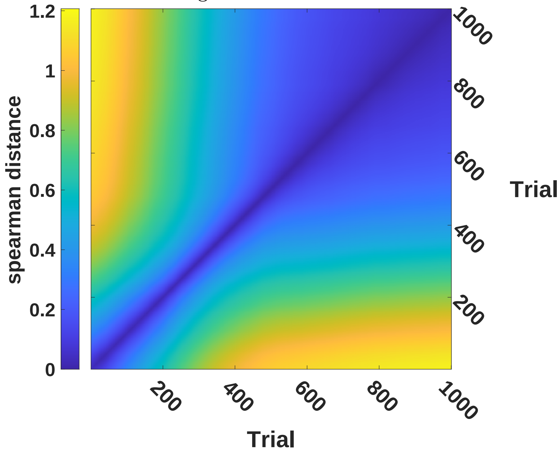
spike orders together Distance Matrix Averaged on 40 Simulations
